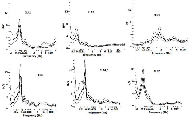
fig. 5. H/V curves of all stations. All the curves are obtained by fulfilling the criteria for clear curve and peak, bold-line is the H/V curve, lower and upper narrow lines indicate upper and lower bound of standard deviation.
