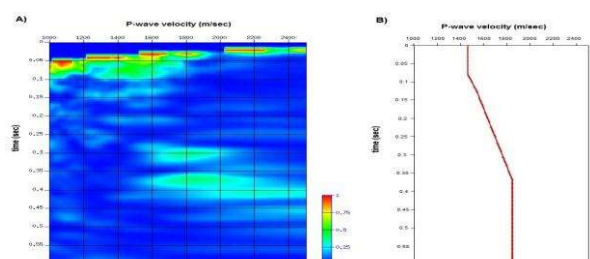
fig.2 - Semblance plot with panel at middle (A) and (B) stacking velocity function of cdp gather 750 from Colonia seismic reflection investigation (P-wave) (modified from Riccomini et al., 2011).
