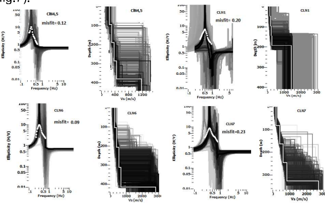
Figure 9. Inversion profiles and misfit values for CLN4,5 , CLN1 ,CLN6 and CLN7. Lowest misfit model profile of VS is shown in white for all the stations.
