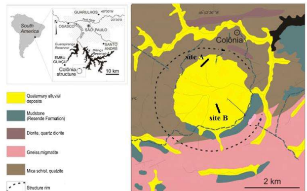
fig. 1. Location (left) and geological map of the Colonia structure. The black thick lines indicates the locations of MASW tests while thin line indicate reflection line. (modified from Riccomini et al., 2011).
