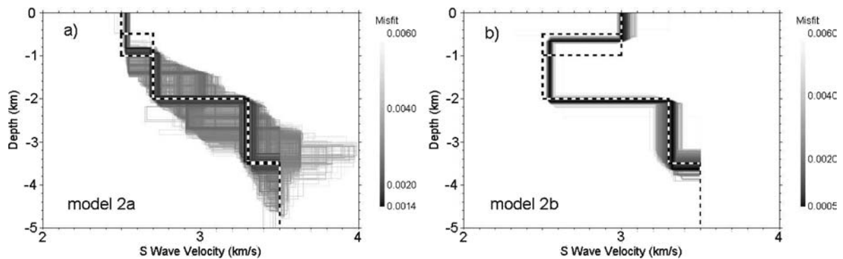
Figure 6. The good inverted models of group 2 (thickness variation in the first and second layers) in the inversion mode 1.
