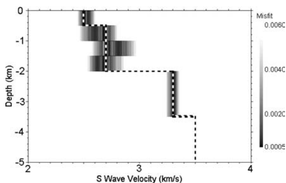
Figure 8. The good inverted models of a synthetic test in the inversion mode 2 to check the convergence of the HGA algorithm.
