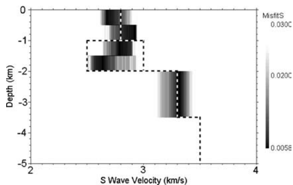
Figure 12. Inversion mode 3 with smoothness constraint in the shallow four layers down to 2 km only. The good inverted models in grayscale of \text{misfitS} (Q_u + 0.007Q_{\text{smooth}}) have smoothness <0.2 km/s. Synthetic data are from model 1dm in Figure 10d.
