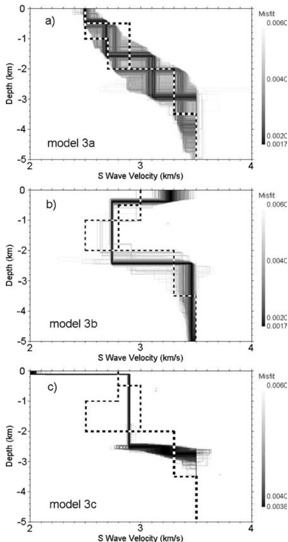
Figure 7. The good inverted models of group 3 (thickness and S velocity variation in the first and second layers) in the inversion mode 1.
