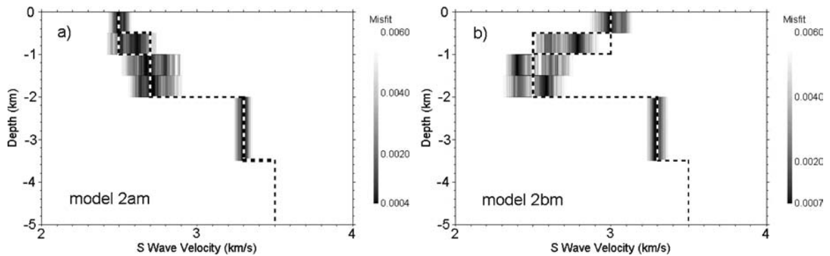
Figure 10. The good inverted models of group 2 (thickness variation in the first and second layers) in the inversion mode 2.
