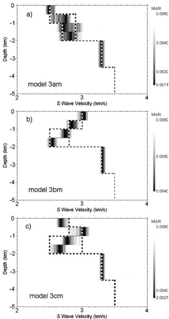
Figure 11. The good inverted models of group 3 (thickness and S velocity variation in the first and second layers) in the inversion mode 2.
